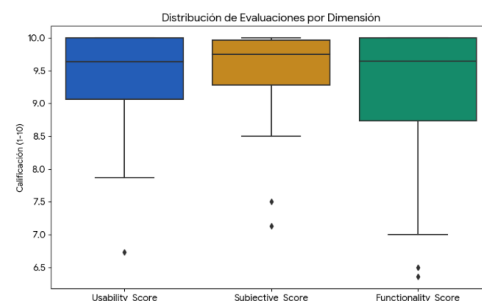
Figure 8: This graph illustrates the variance of the distribution of evaluations by dimension.
